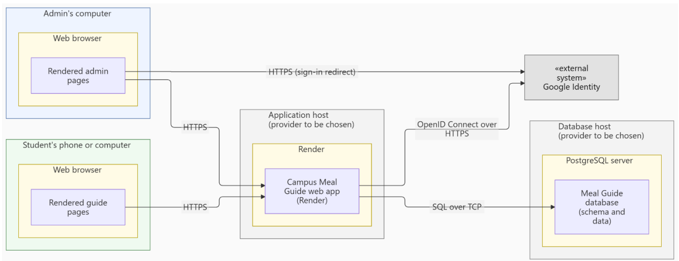
DEPLOYMENT DIAGRAM
