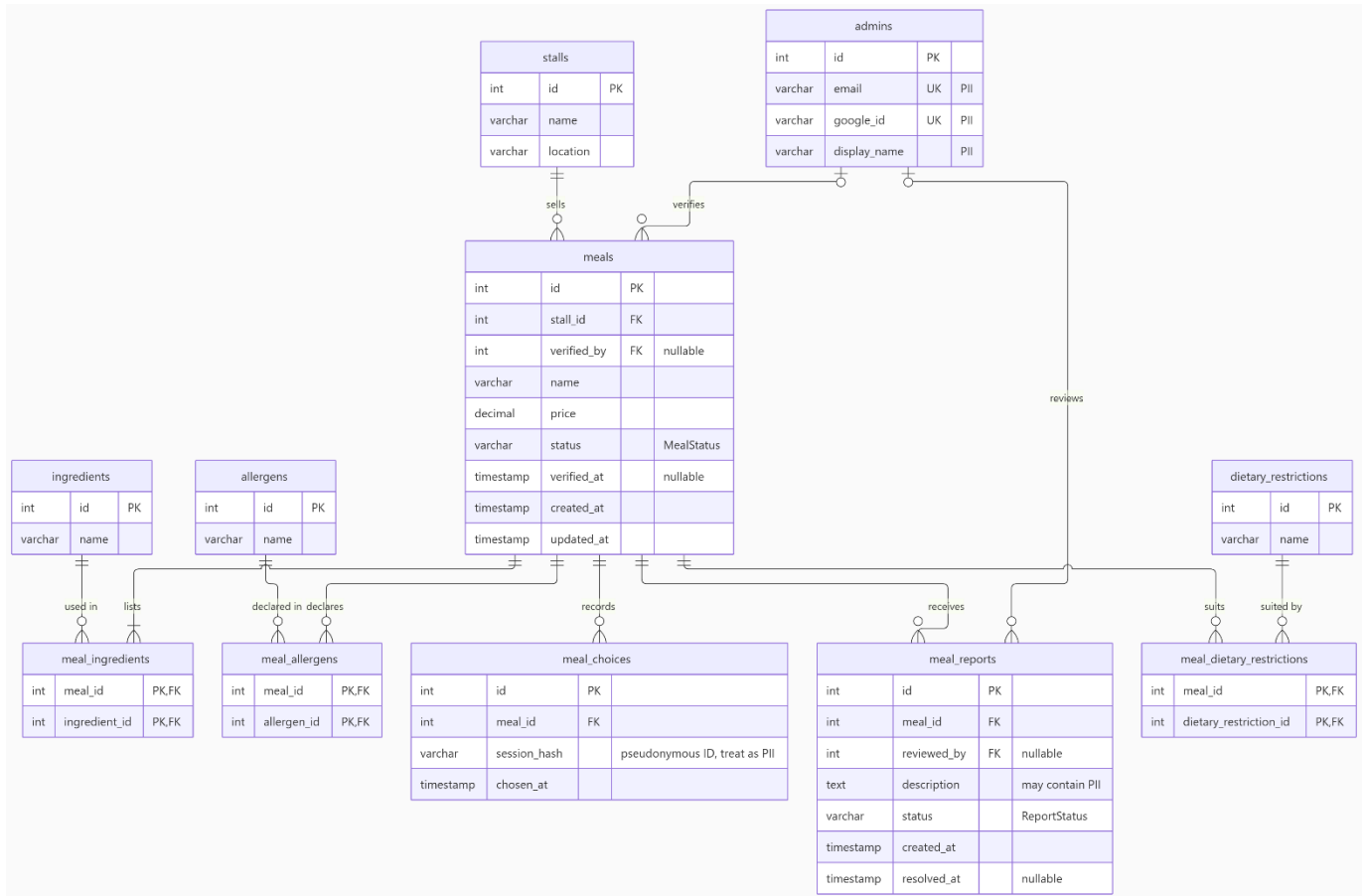
ERD DIAGRAM
