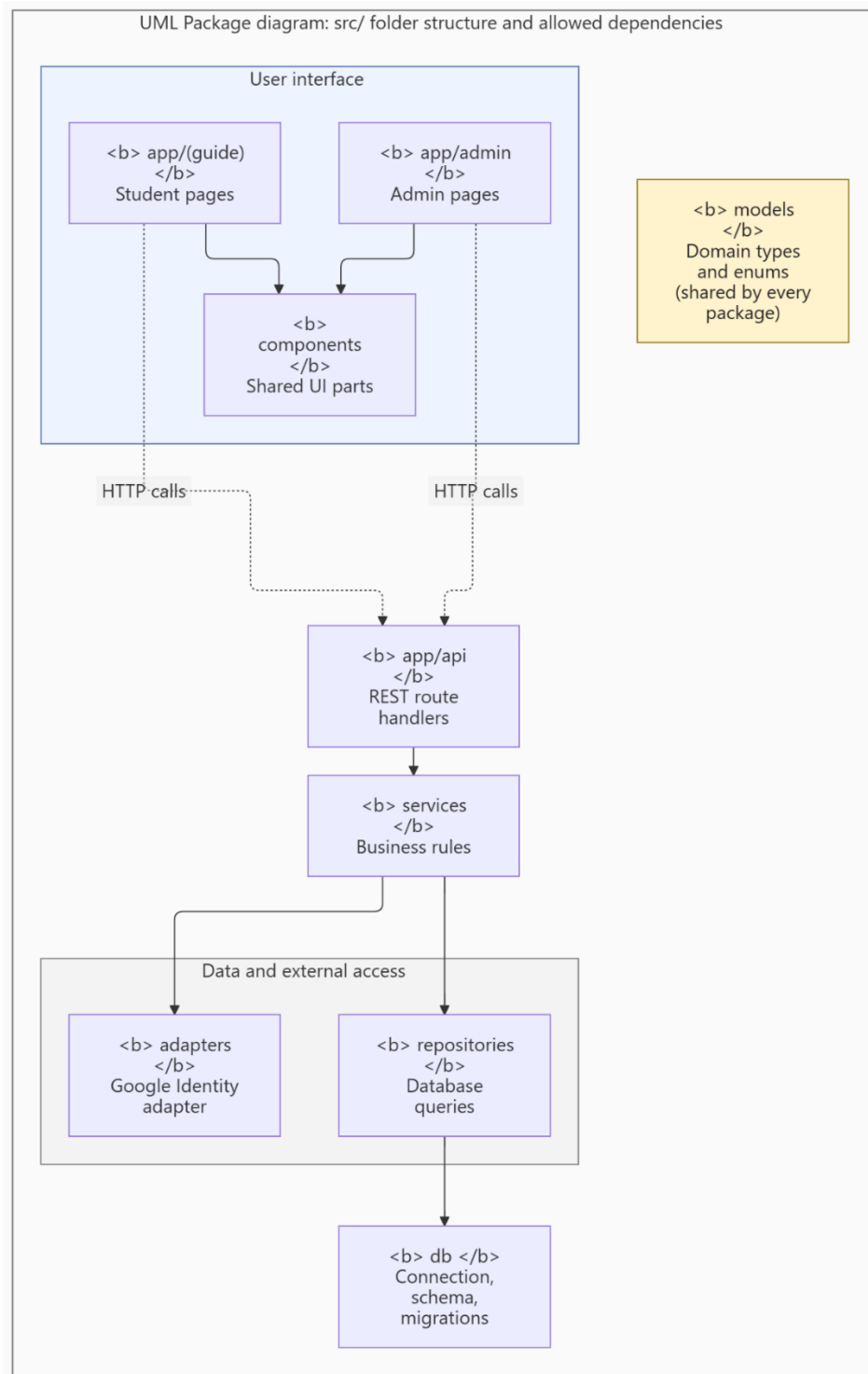
PACKAGES DIAGRAM
