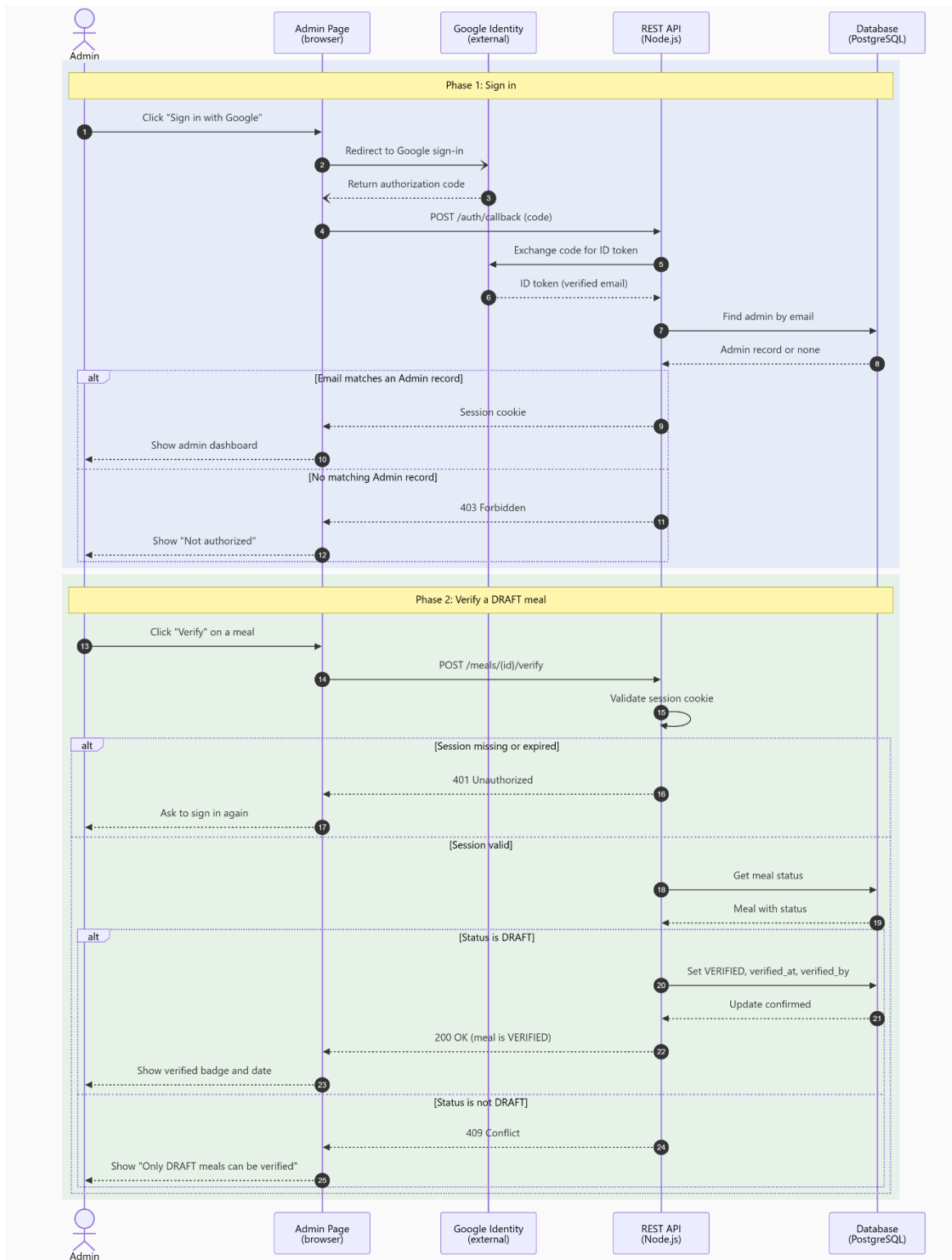
SEQUENCE DIAGRAM
